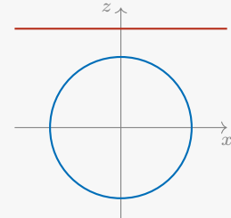
c_1^2 < c_2^2 : kesişmez
