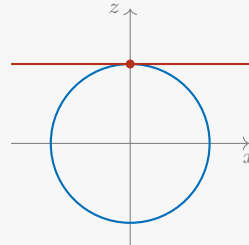
c_1^2 = c_2^2 : tek nokta
